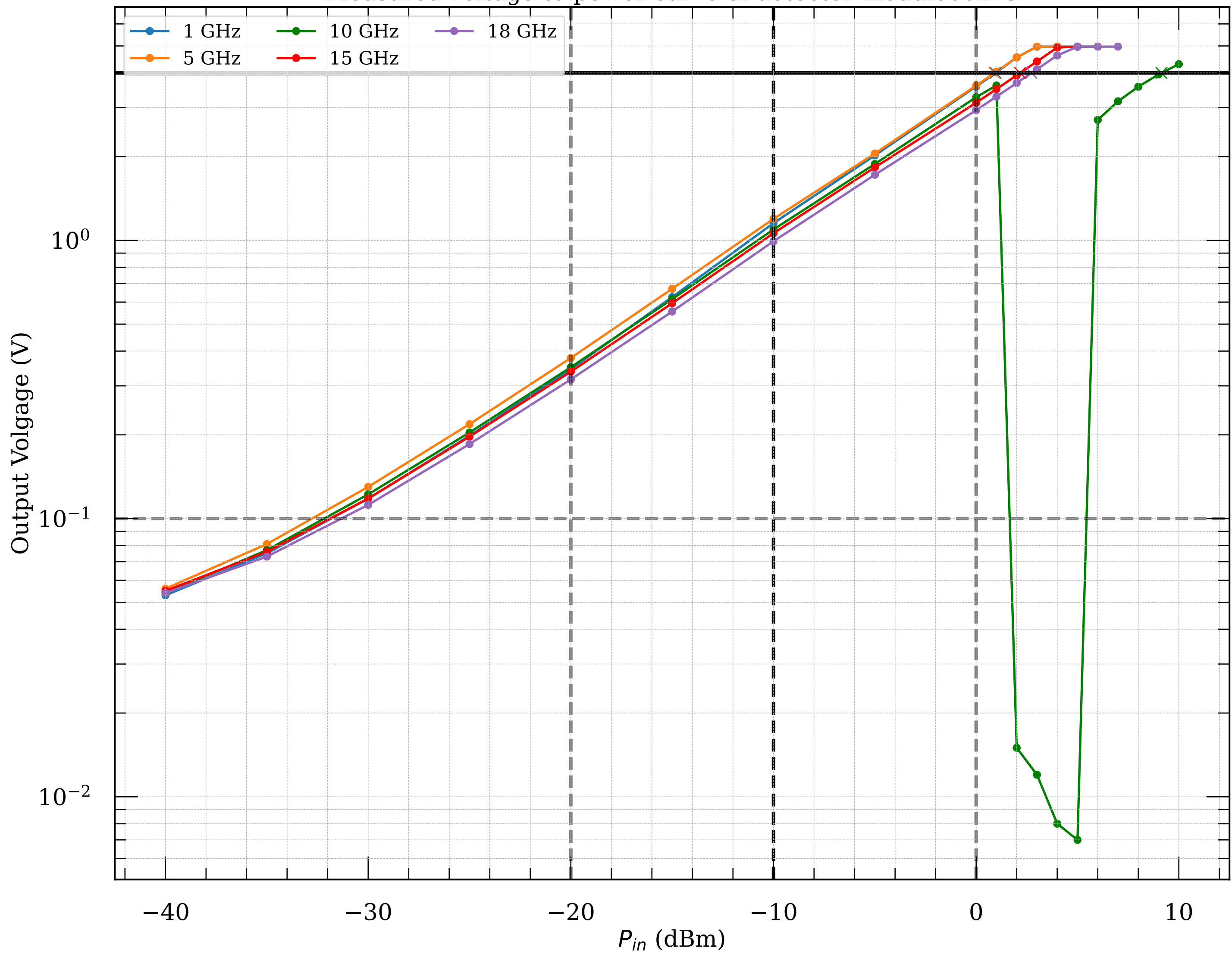
Measured voltage-to-power curve of detector module002v3
